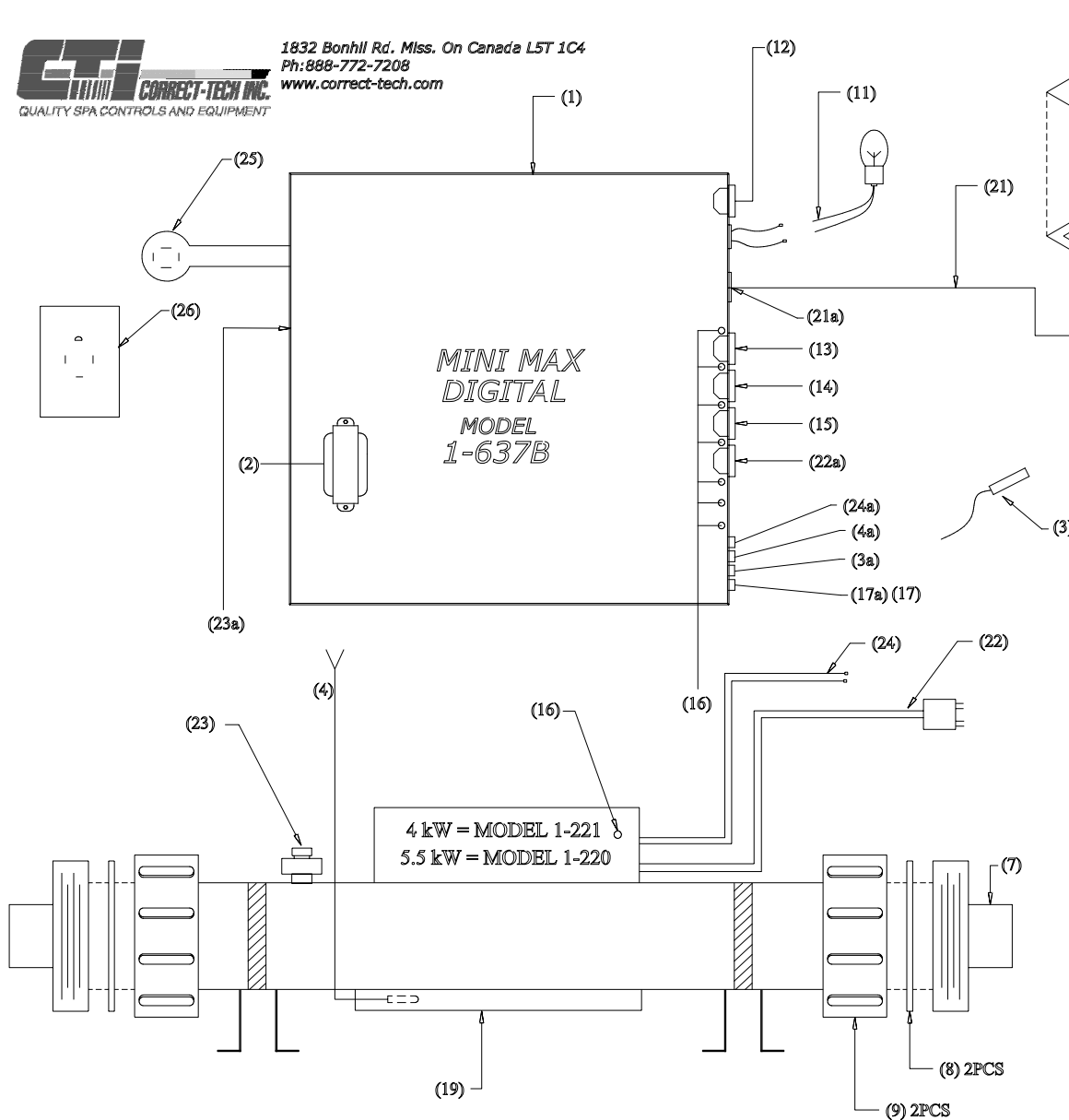
MINI MAX DIGITAL SPA PAK & REMOTE HEATER COMPONENTS DESCRIPTION DWG # 4-30-1204B
